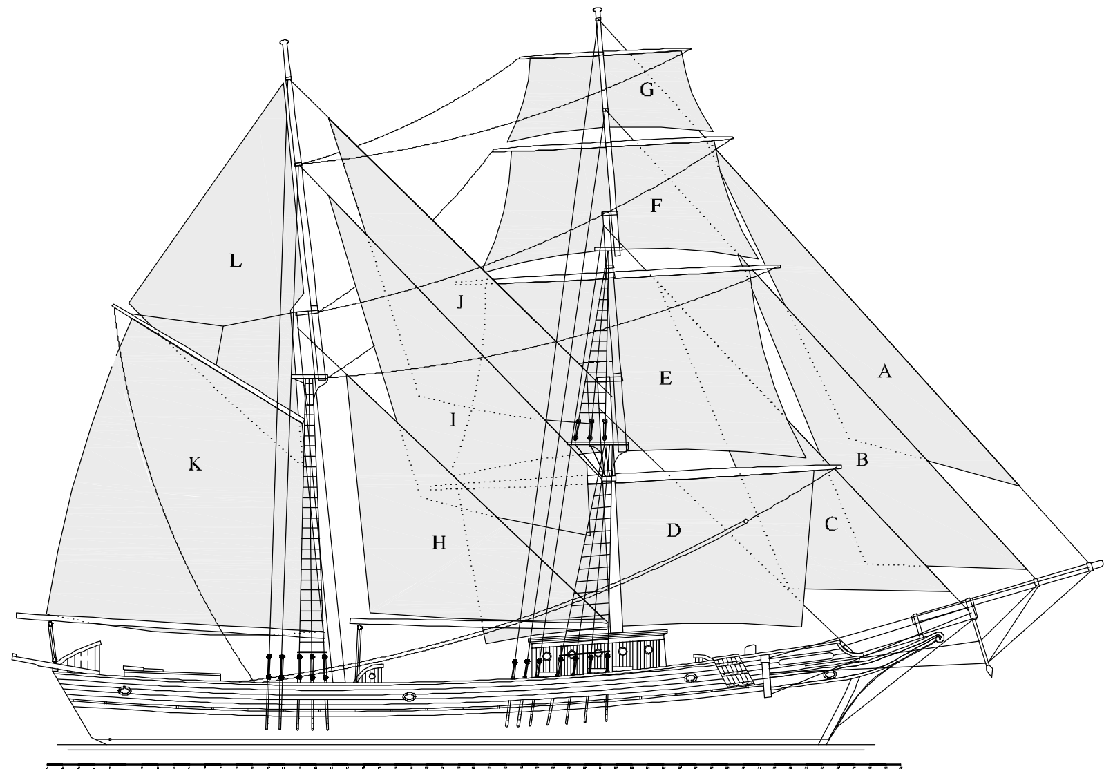
SCHOONERBRIG 'TRES HOMBRES' PINRAIL DIAGRAM
